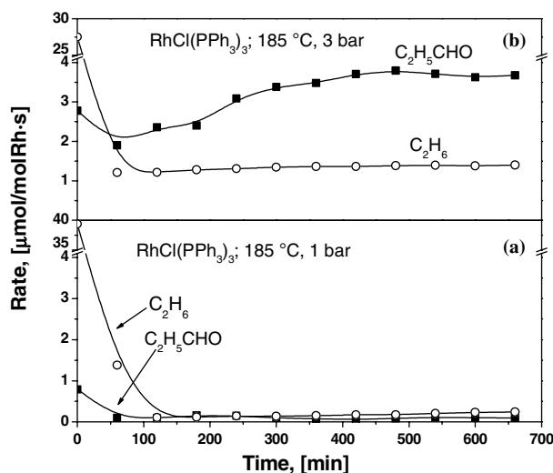
Figure 1. Propanal and ethane formation rates of with time-on-stream over 0.4 g RhCl(PPh 3 ) 3 powder at 185 °C, gas flow rate 3.5 ml/min (a) at 1 bar (b) at 3 bar.
